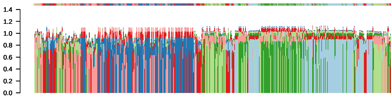
item-consensus k=6
